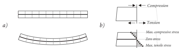
Figure 2: Beam geometry. a) Cross-sectional view of bending deformation. b) Linearly varying stresses through the thickness and neutral axis .
