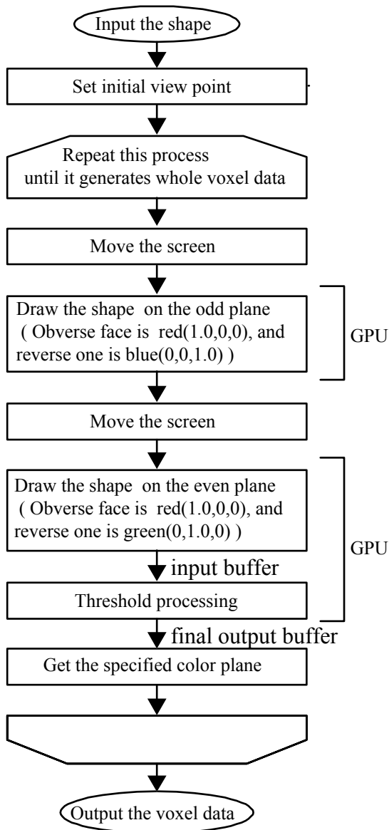
Figure 10. The flow for improving the accuracy of the voxel data
