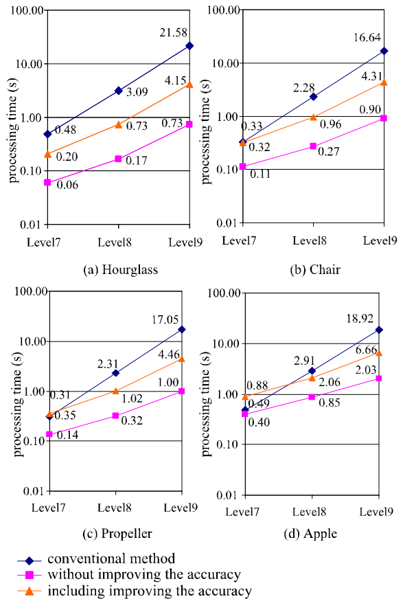
Figure 12. Relation of the generation time to the level
