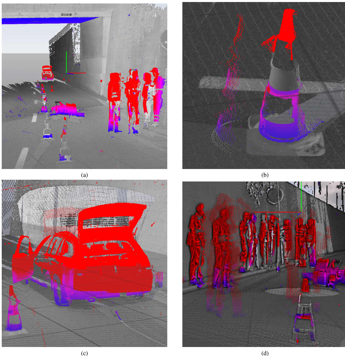
Figure 9: Some classifications inferred by our algorithm. For these images a threshold of 2 cm was used. The blue area on the ceiling in (a) is due to inaccurate registration of the scans and has to be taken care of by choosing an appropriate threshold. The cone in (b) was slightly displaced during scans, allowing at least the artifact from one scan (left) to be completely recognized. c) The car was apparently completely removed for at least one scan, which made it almost completely recognizable. Note the slight shadow of the tailgate, indicating that this car was slightly displaced also present in a second scan. d) A group of people that was present at roughly the same place during different scans. Note that parts of the group in the background could not be classified, since they were shadowed by other people closer to the scanners (Shading was added to improve geometric structure perception).
