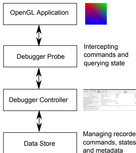
Figure 1: Architectural overview of GLDebug.
