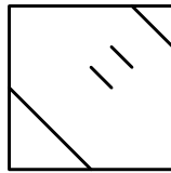
Figure 2: The support of the layered permuton associated with the permutation 43215687 as in the proof of Lemma 6. The origin of the coordinate system is in the bottom left corner.
