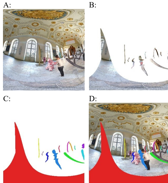
Figure 3. Pruning and clustering; A: input view (sequence Museum), B: view after pruning, C: preserved pixels after clustering, D: preview of clusters within input view.
