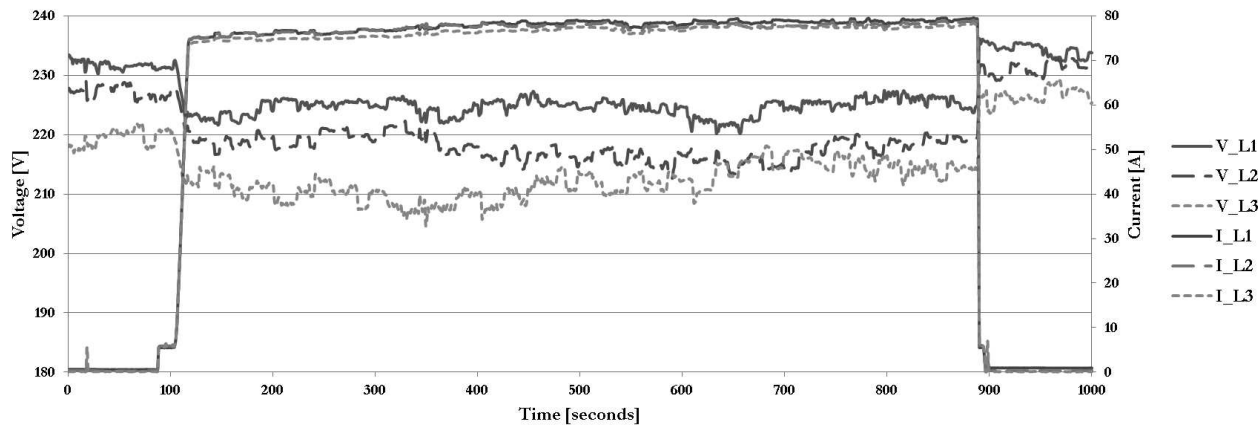
Fig. 1 Typical voltage a current profiles when EV DC charging 50 kW
