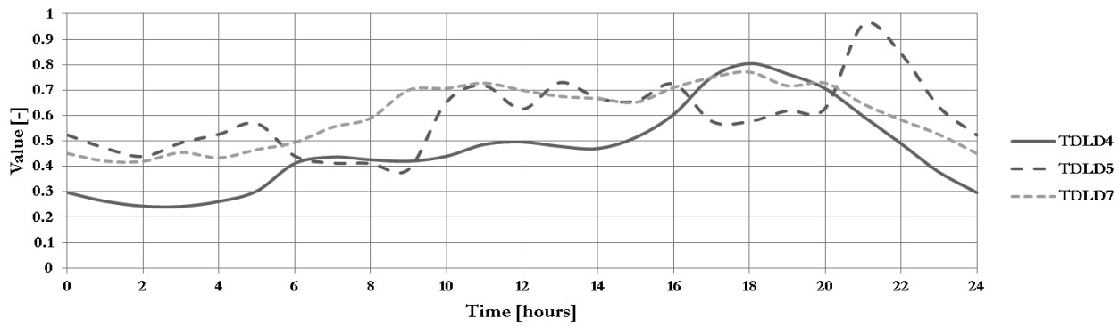
Fig. 3 Typified daily load diagrams for household active power consumptions
