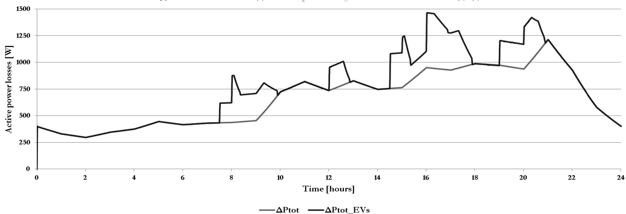
Fig. 9 Total active power losses on cable lines without and with EV's charging
