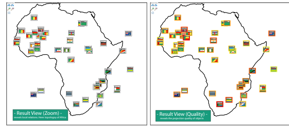
Figure 6: Result View. Rotation, zooming and panning reveals data subspaces (here: Africa). On the right the projection quality can be seen by colored outlines (green to red).
