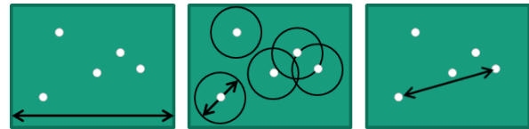
Figure 2: Object Alignment Strategies. Left: absolute . Centre: orbital . Right: relative .
