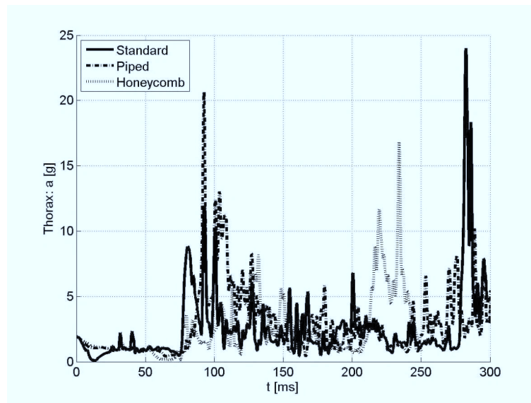
Fig. 8. Comparison of driver thorax acceleration for different tram fenders
