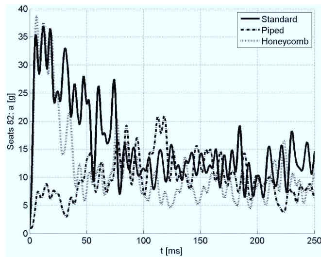
Fig. 12. Seat acceleration for bullet tram
