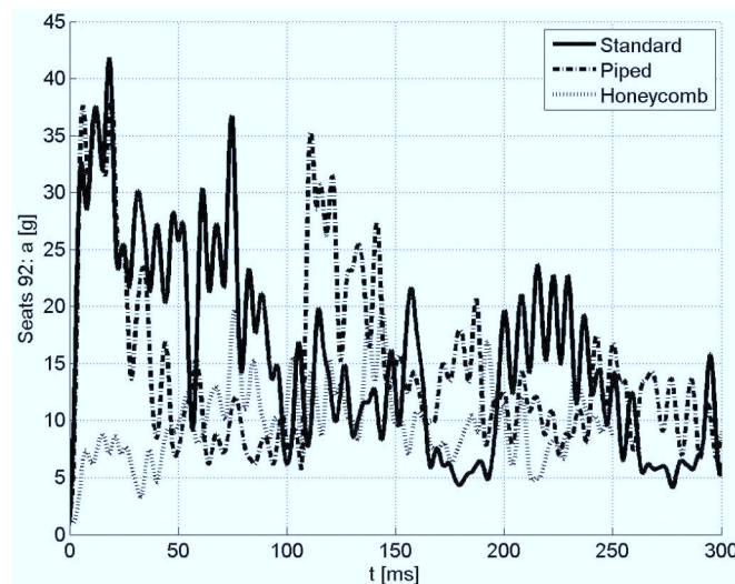
Fig. 13. Seat acceleration for target tram
