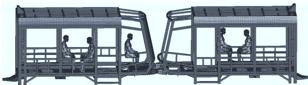
Fig. 9. Impacting trams including driver and passengers
