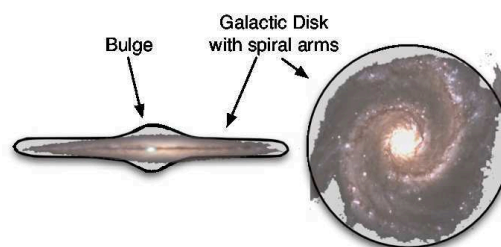
Figure 3: Generic Galaxy Shape. On the left is the so-called edge-on view ( 90^\circ ). The dust is concentrated along a galaxy's equatorial region. Compared to the right, which is often referred to as face-on view ( 0^\circ ), where the dust is concentrated along the spiral arms.
