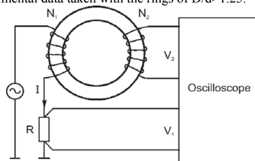
Fig. 1. The unit to measure power losses in SMC materials
