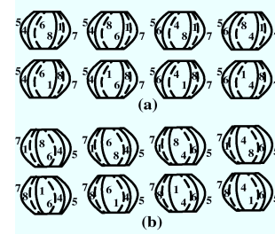
Fig. 10 - Cases (a) and (b) and the 16 sub-cases
