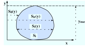
Fig. 5 - Notations used for a silhouette.
