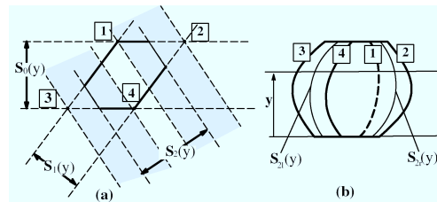
Fig. 6 - The condition for the compatibility of S_2(y)
