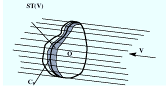
Fig. 3 - The annular strip ST(V) and the curve C_V
